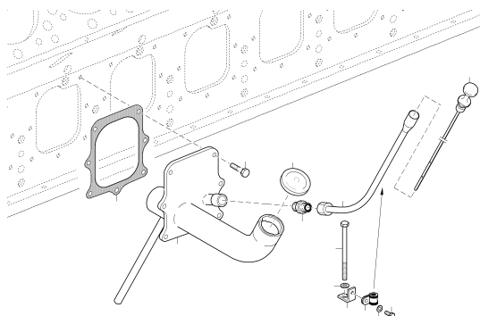
OIL FILLER NECK UPC.06G04 1388
